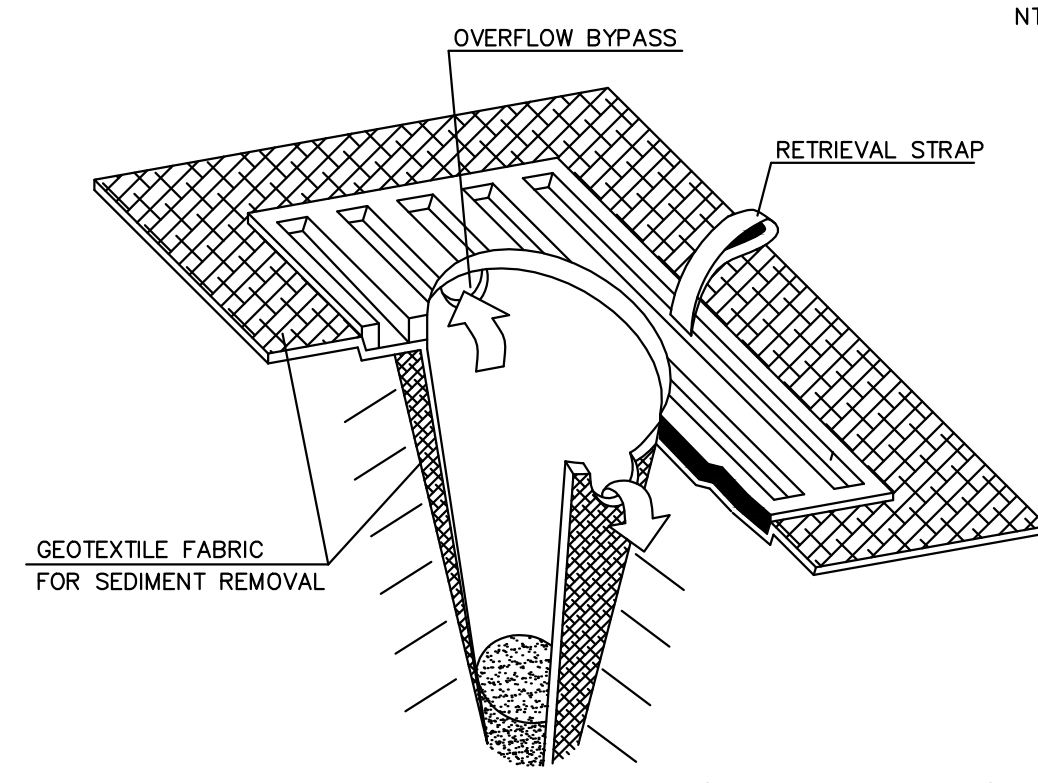
STORM DRAIN PROTECTION INSERT DETAIL NOT TO SCALE
