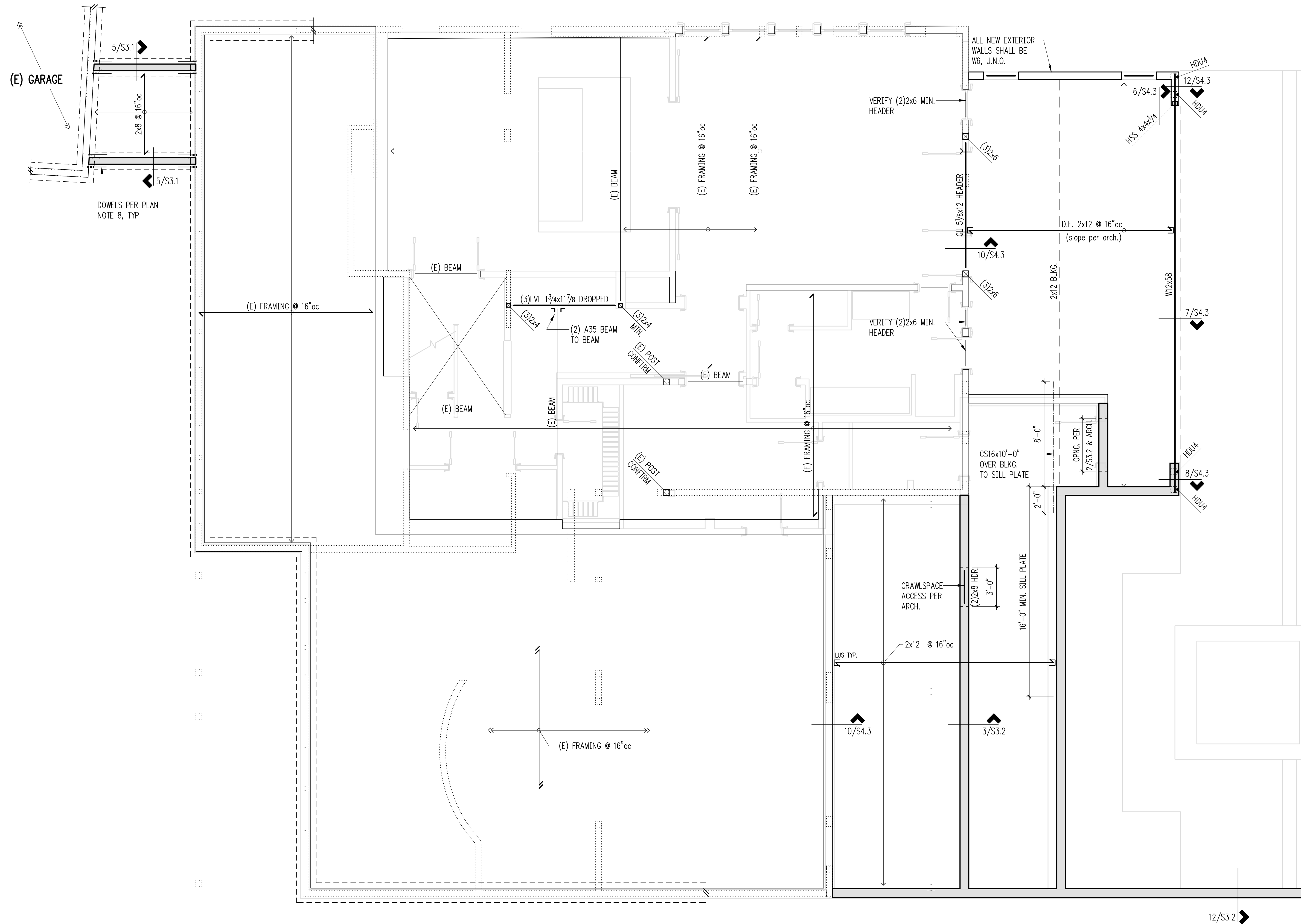
Main Floor Framing Plan Scale: 1/4" = 1'-0"
