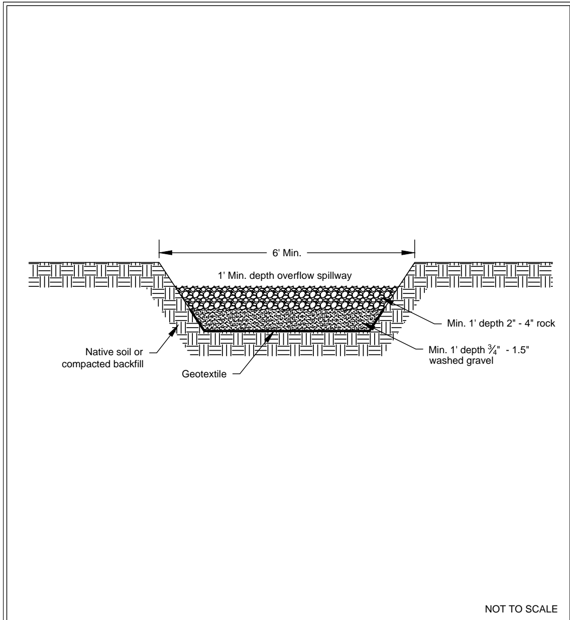
Figure II-4.2.17 Sediment Trap Outlet
