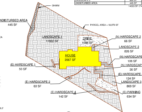
2 SITE AREAS 1/32" = 1'-0"
