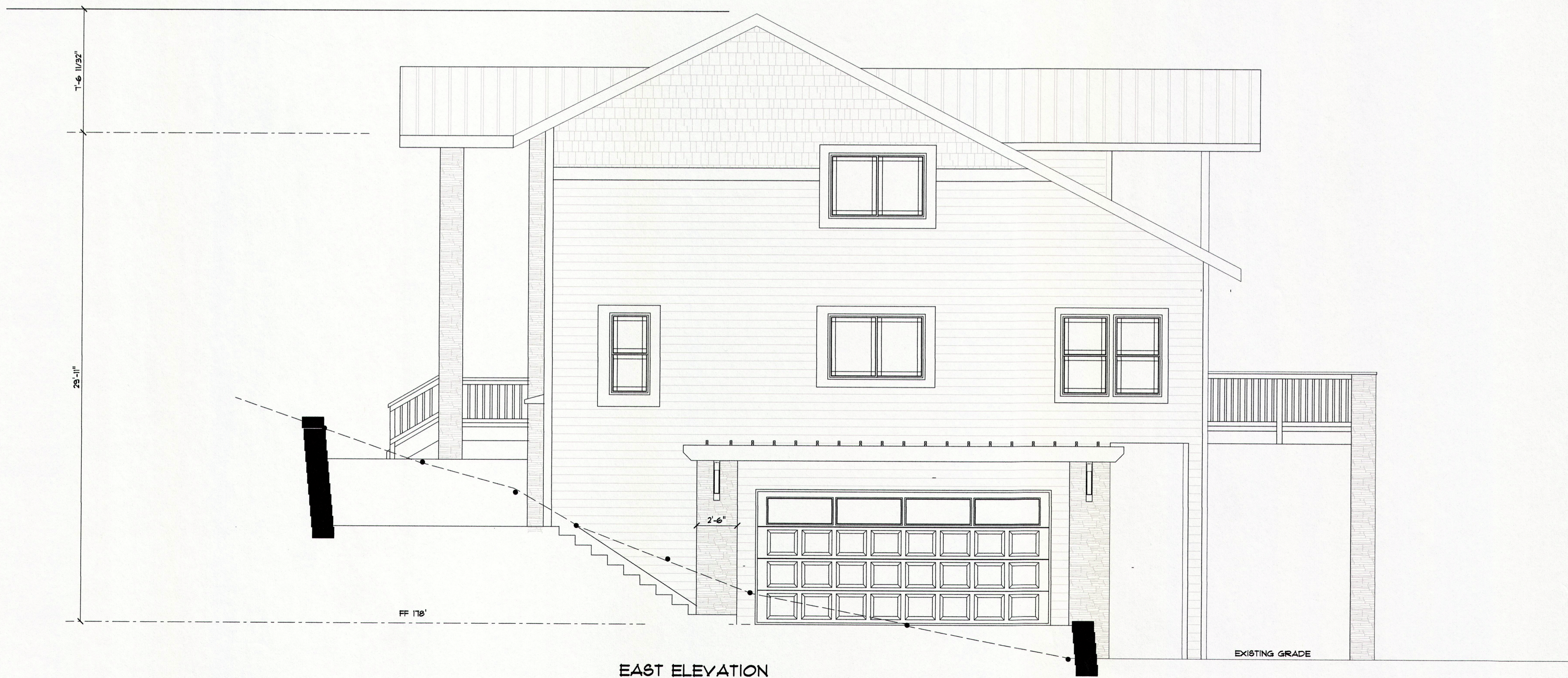
EAST ELEVATION
