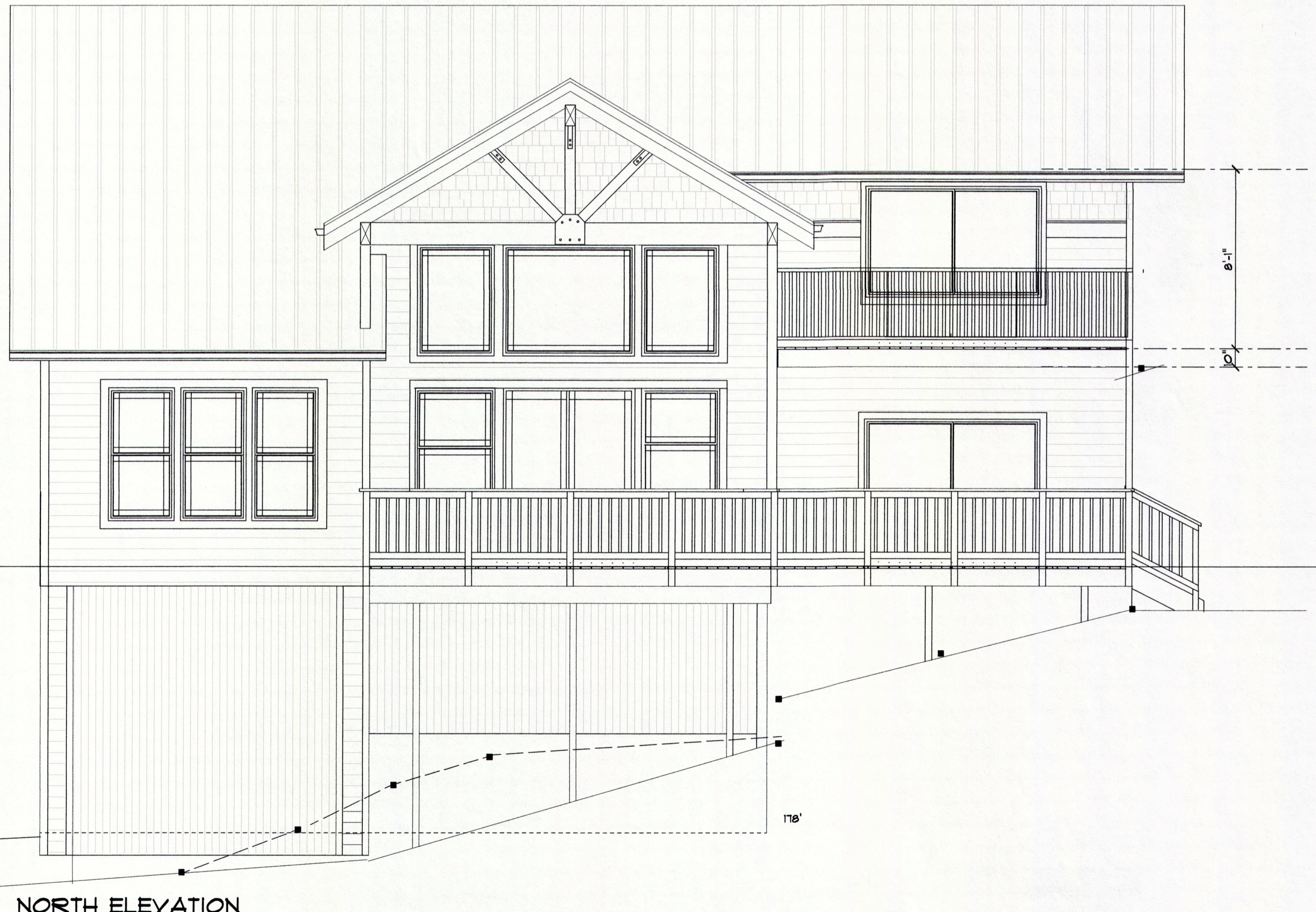
NORTH ELEVATION
